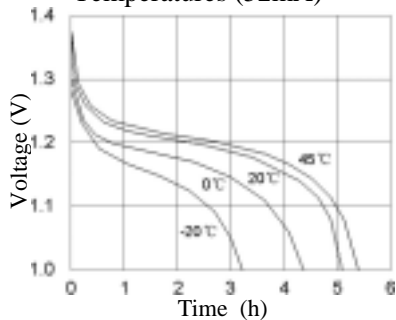
Discharge Curve at Various Temperatures (52mA)
