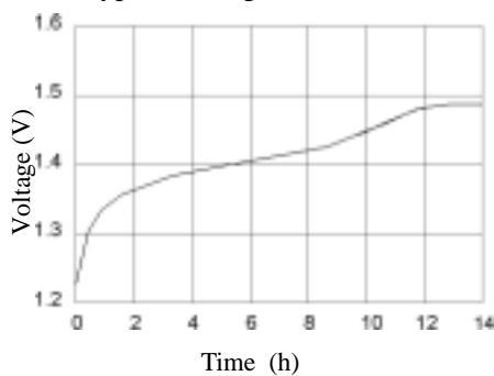
Typical Charge Curve (23mA)
