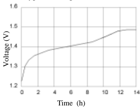
Typical Charge Curve (17mA)
