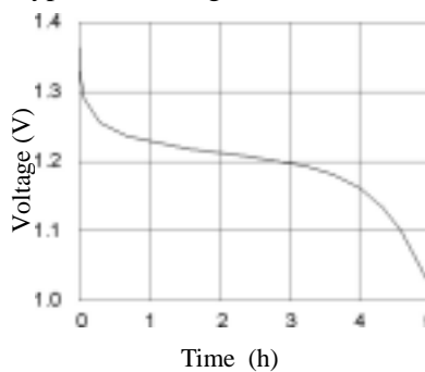
Typical Discharge Curve (34mA)
