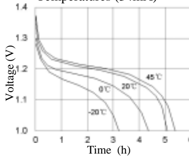
Discharge Curve at Various Temperatures (34mA)
